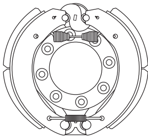
TRACTOR BRAKE
