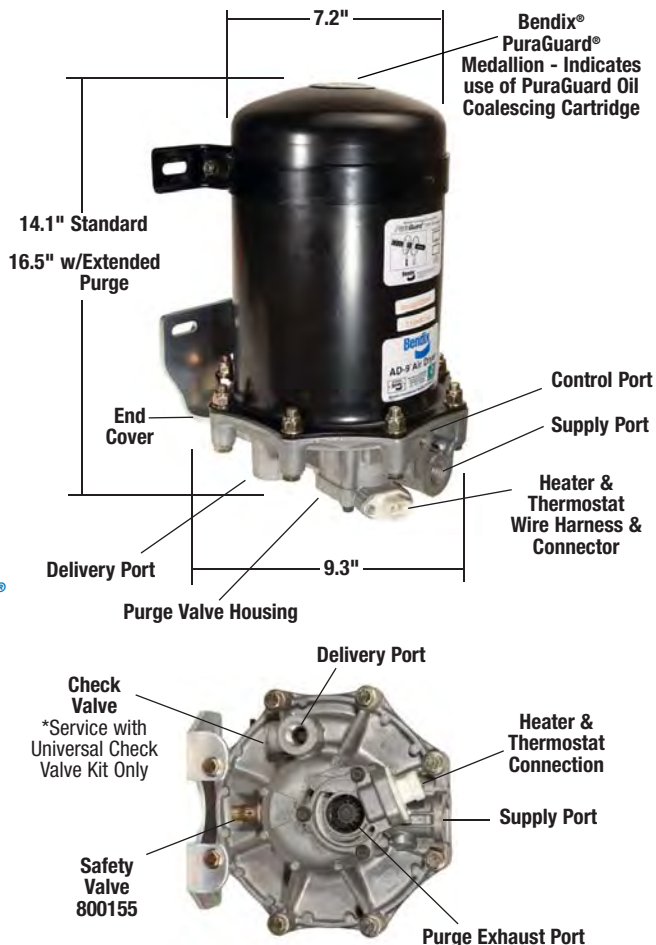
New Style End Cover
