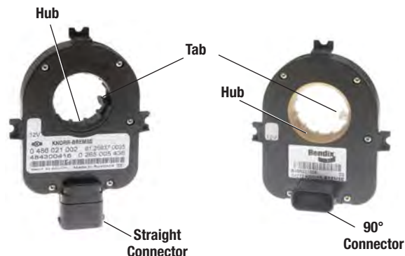
Bendix® SAS-60™ Steering Angle Sensor
