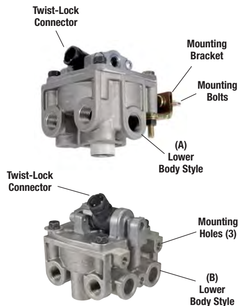
Bendix® ATR-6™ Traction Relay Valve
