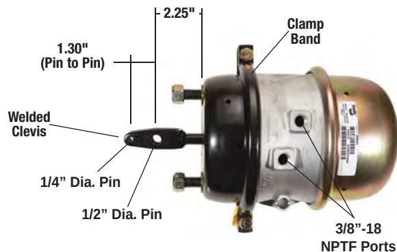
Bendix® EverSure® Spring Brake with Welded Clevis
