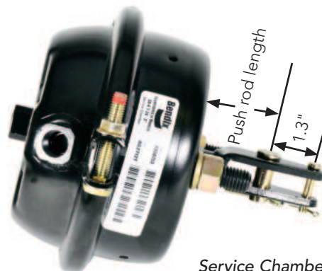
Service Chamber with welded clevis
