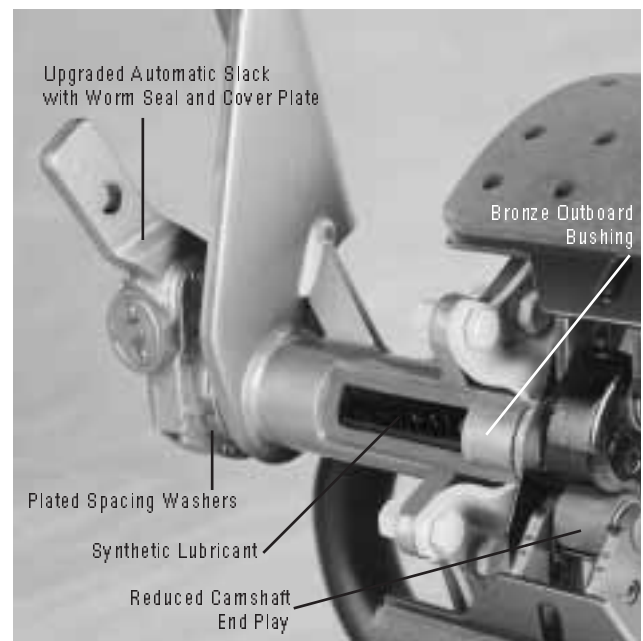
The Bendix® LMS™ Brake Package featuring Bendix® ES™ Wide Brakes — the original thick lining brake.
