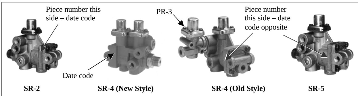
Figure 1 - Valve Identification
