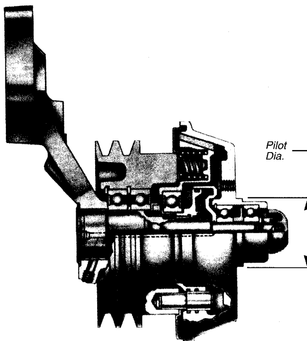
FD-3 TorqueMaster (2.56" Pilot Diameter)
