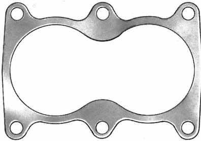
CYL. BLK. GASKET Pc. No. 241560 FOR TF-600 & 700 COMPR.
