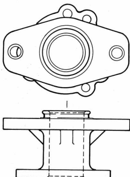
MOUNTING PLATE 245203
