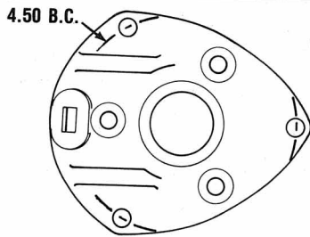
TOP VIEW OF MOUNTING PLATE
