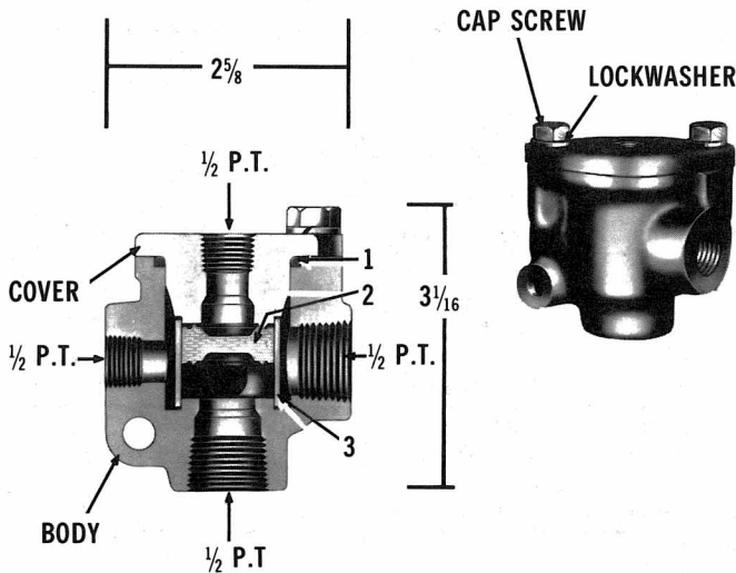
DC-2 DOUBLE CHECK VALVE PC. NO. 223869
